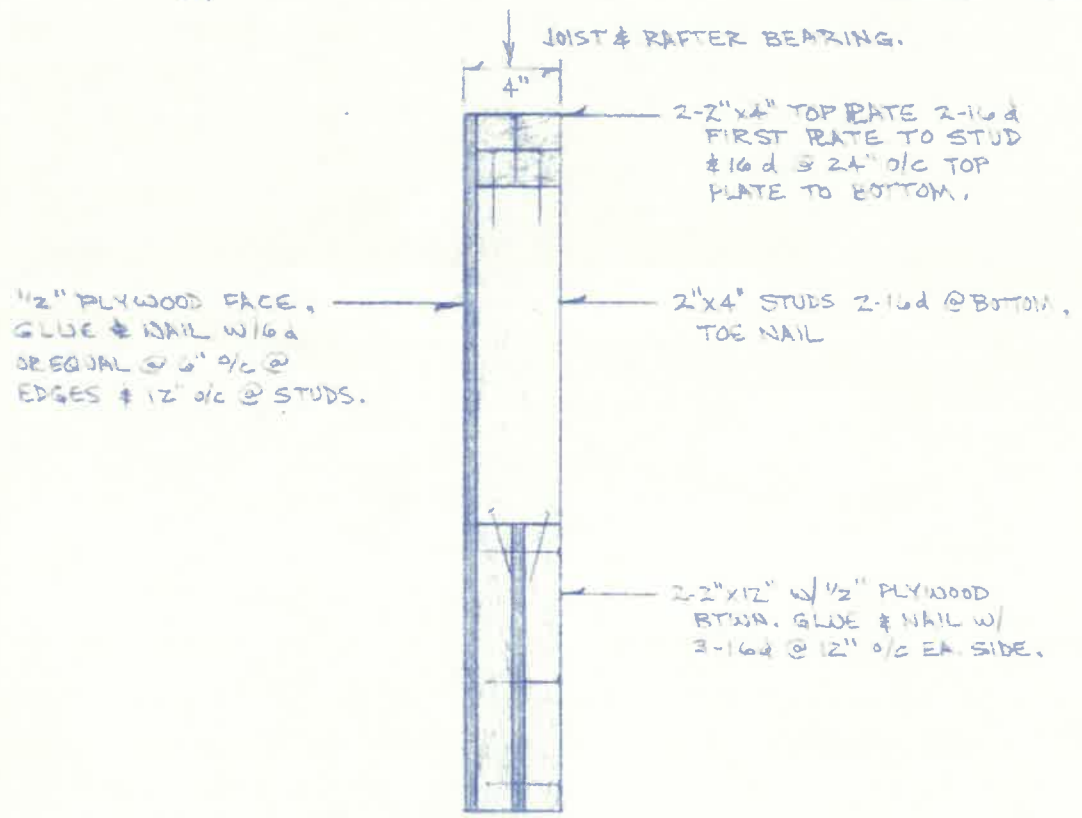
SECTION A-I 1 1/2" = 1'-0"
